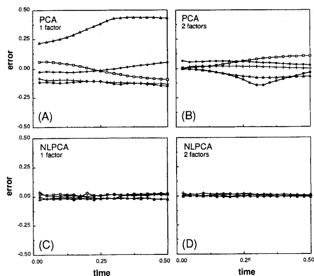
Figure 8. Errors in reproducing data for batch run in Figure 7 from feature space representations.
