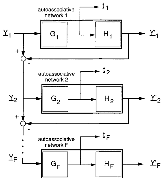
Figure 3. Sequential determination of nonlinear factors by training F networks with one bottleneck node each.
