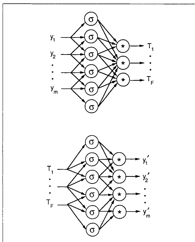
Figure 1. Networks implementing mapping and demapping functions.
