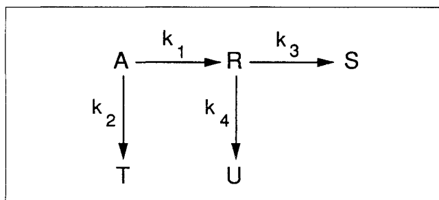
Figure 6. Reaction network for example 2.
