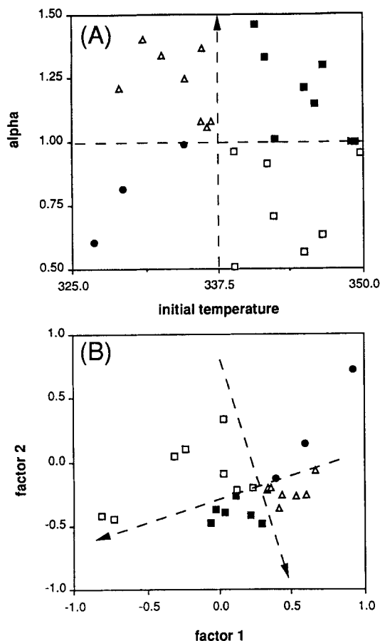
Figure 9. Underlying factors by NLPCA in example 2.
