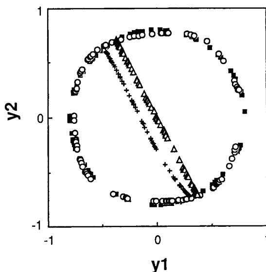
Figure 4. Reconstructed data from one factor, example 1.
