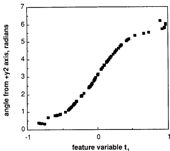
Figure 5. Feature variable derived by NLPKA, example 1, showing discovery of a feature analogous to underlying parameter \theta .
